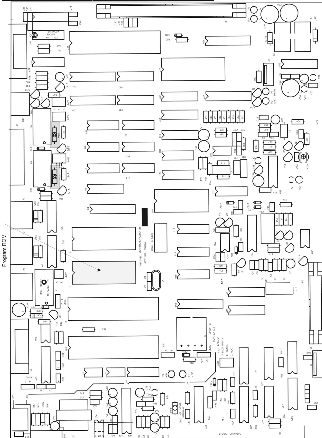
Figure 1. Model 1084A/B/C Main Board
